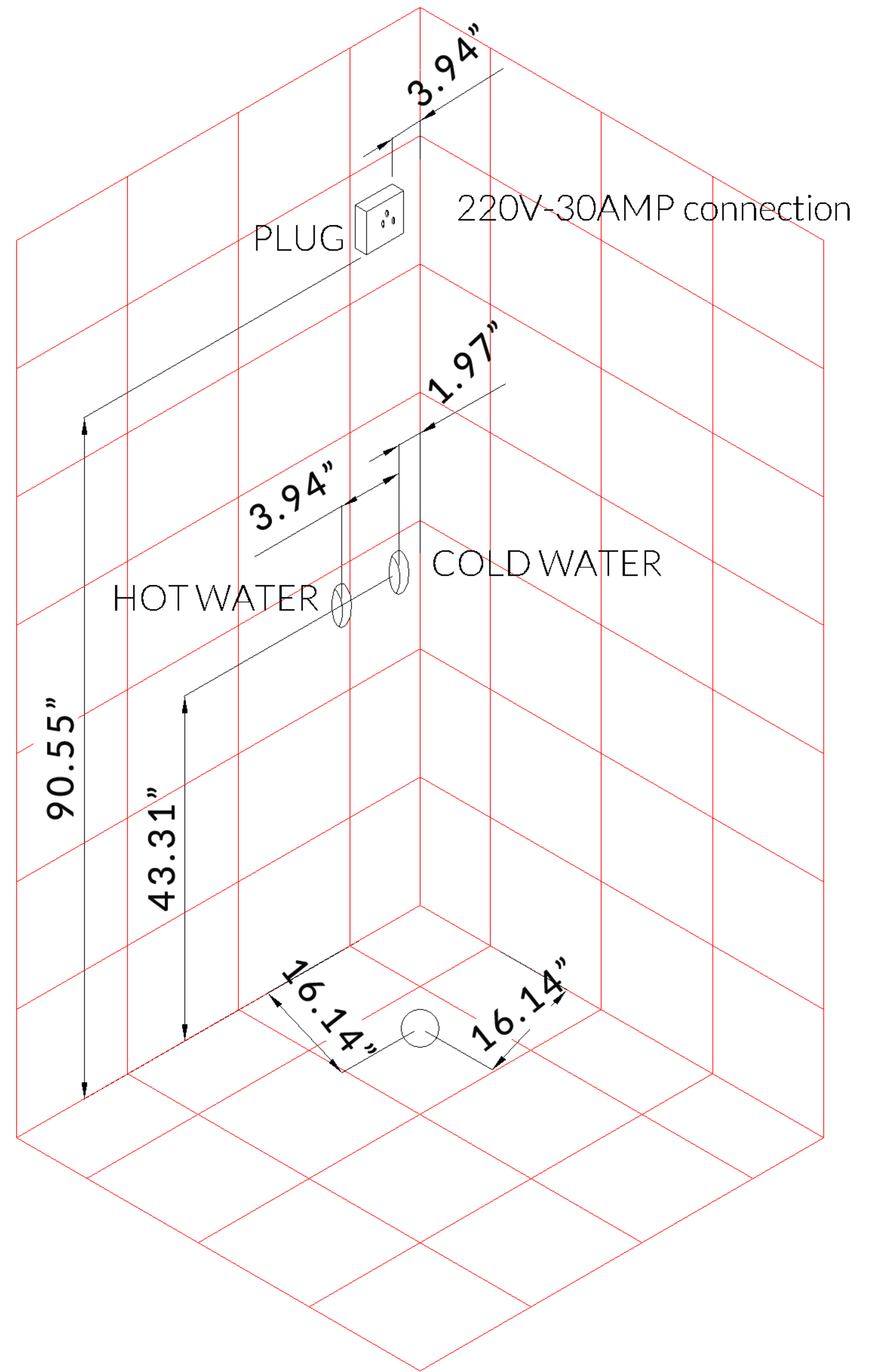
DZ961F8 INSTALLATION (LEFT) DIMENSIONS: 59" x 35" x 89"
